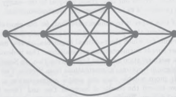
Figure 1: The best single-edge addition is to double the lower edge.
